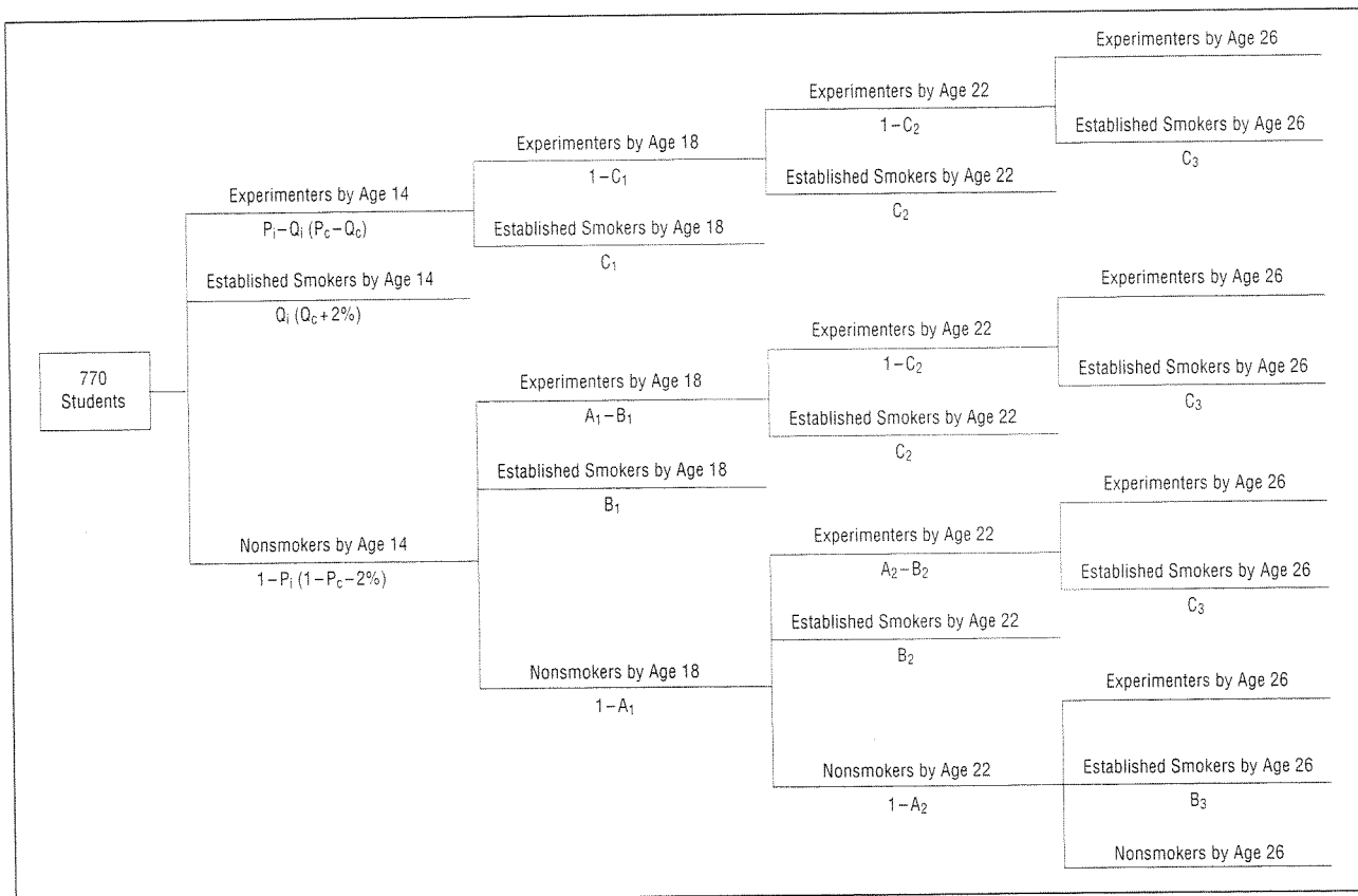
Smoking progression model. Parameters in parentheses indicate control scenario. All ages are given in years.
